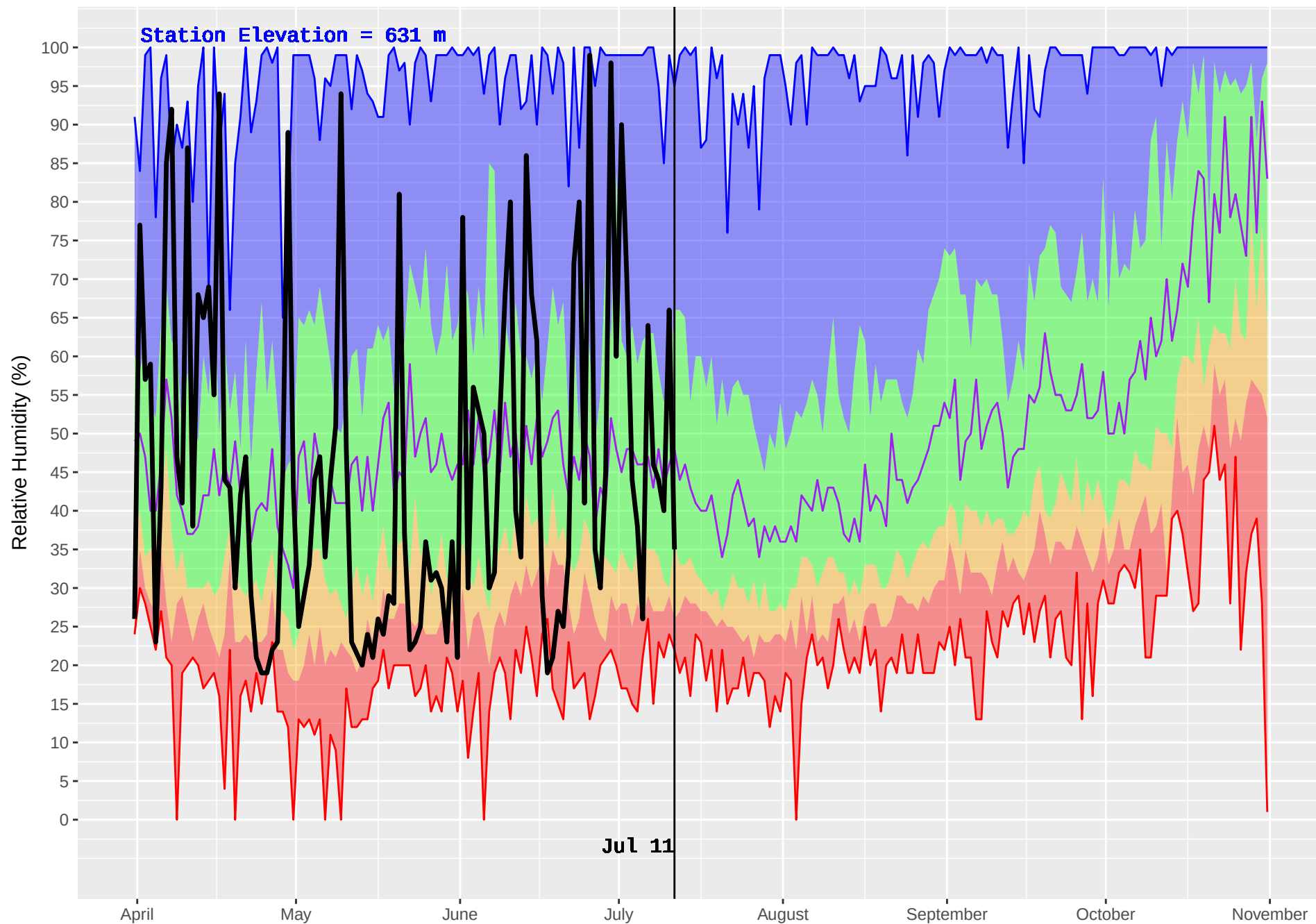
EAST BARRIERE (243) : Historical (1978–2016) and Current (2018) Noon Relative Humidity
