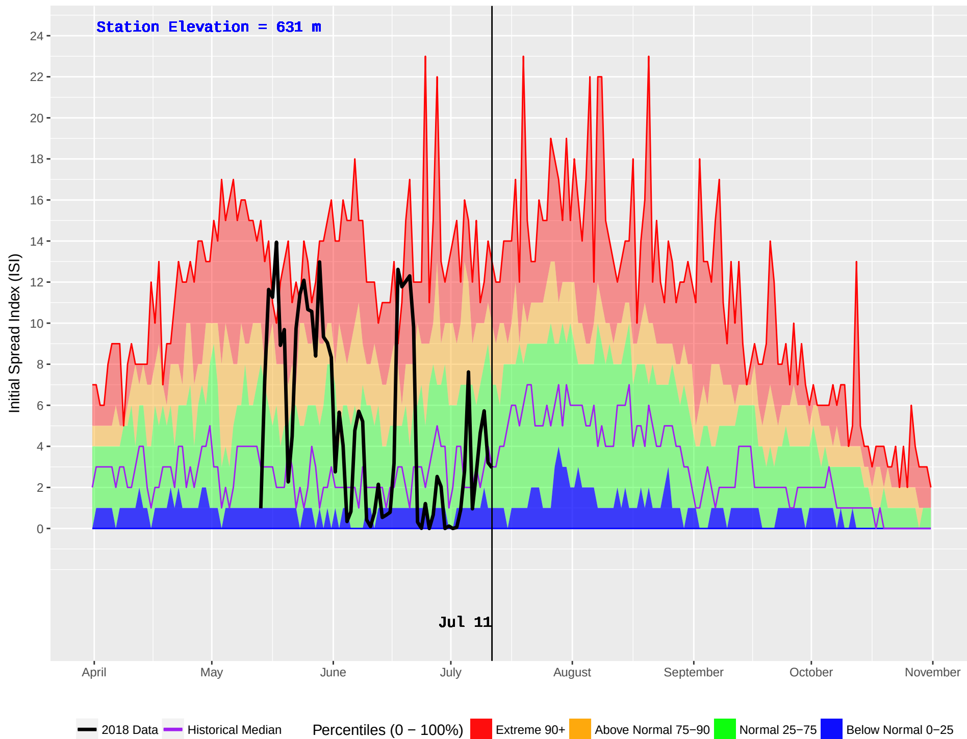
EAST BARRIERE (243) : Historical (1978–2016) and Current (2018) Noon Initial Spread Index (ISI)
