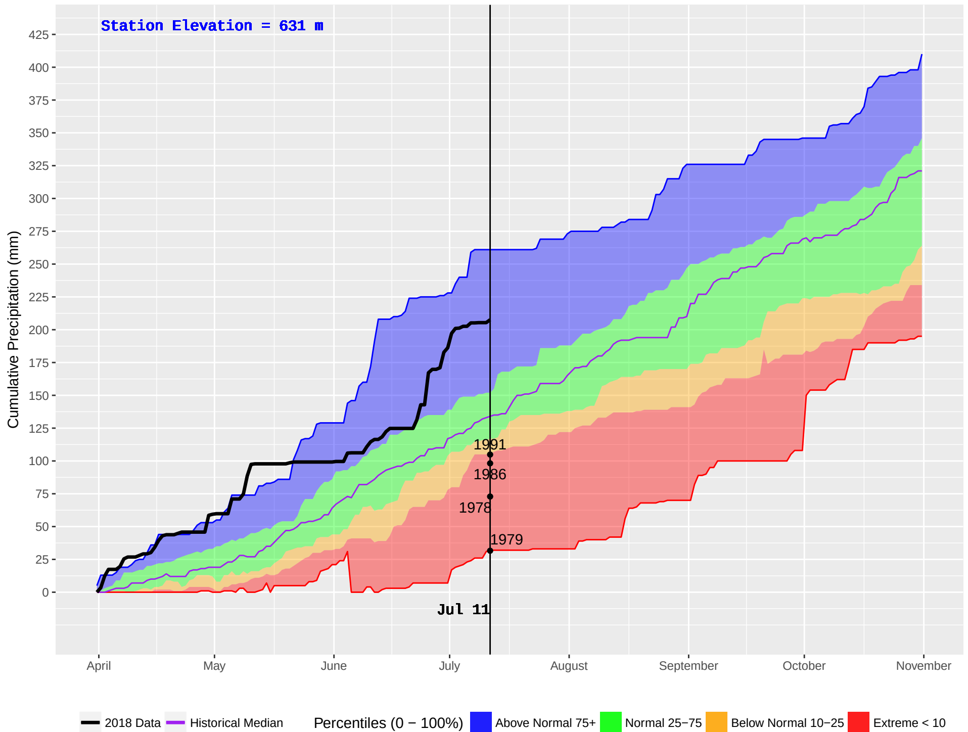
EAST BARRIERE (243) : Historical (1978–2016) and Current (2018) Noon Cumulative Precipitation
