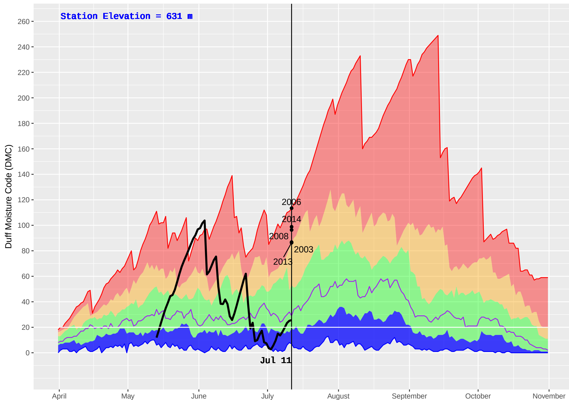
EAST BARRIERE (243) : Historical (1978–2016) and Current (2018) Noon Duff Moisture Code (DMC)
