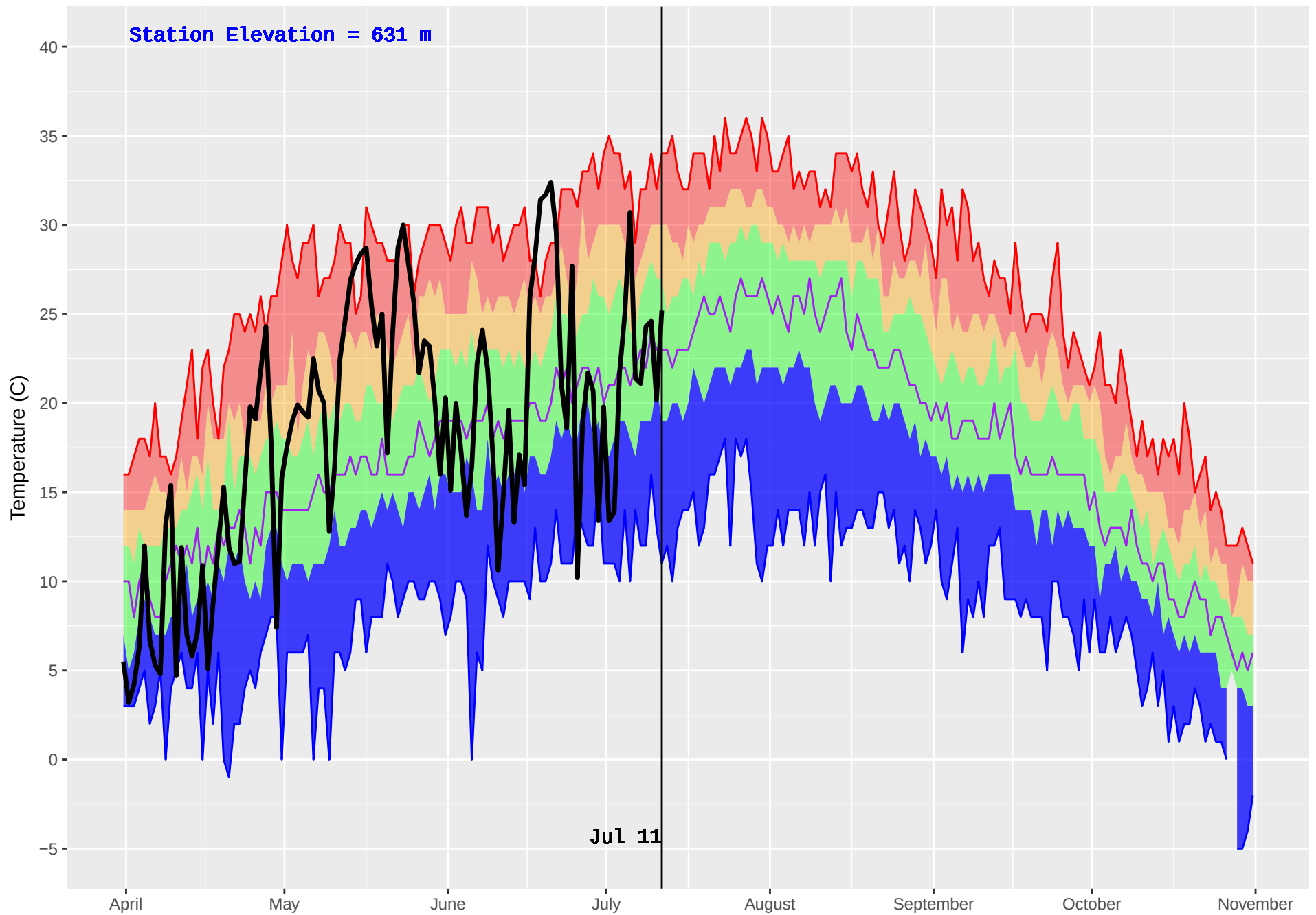
EAST BARRIERE (243) : Historical (1978–2016) and Current (2018) Noon Temperature
