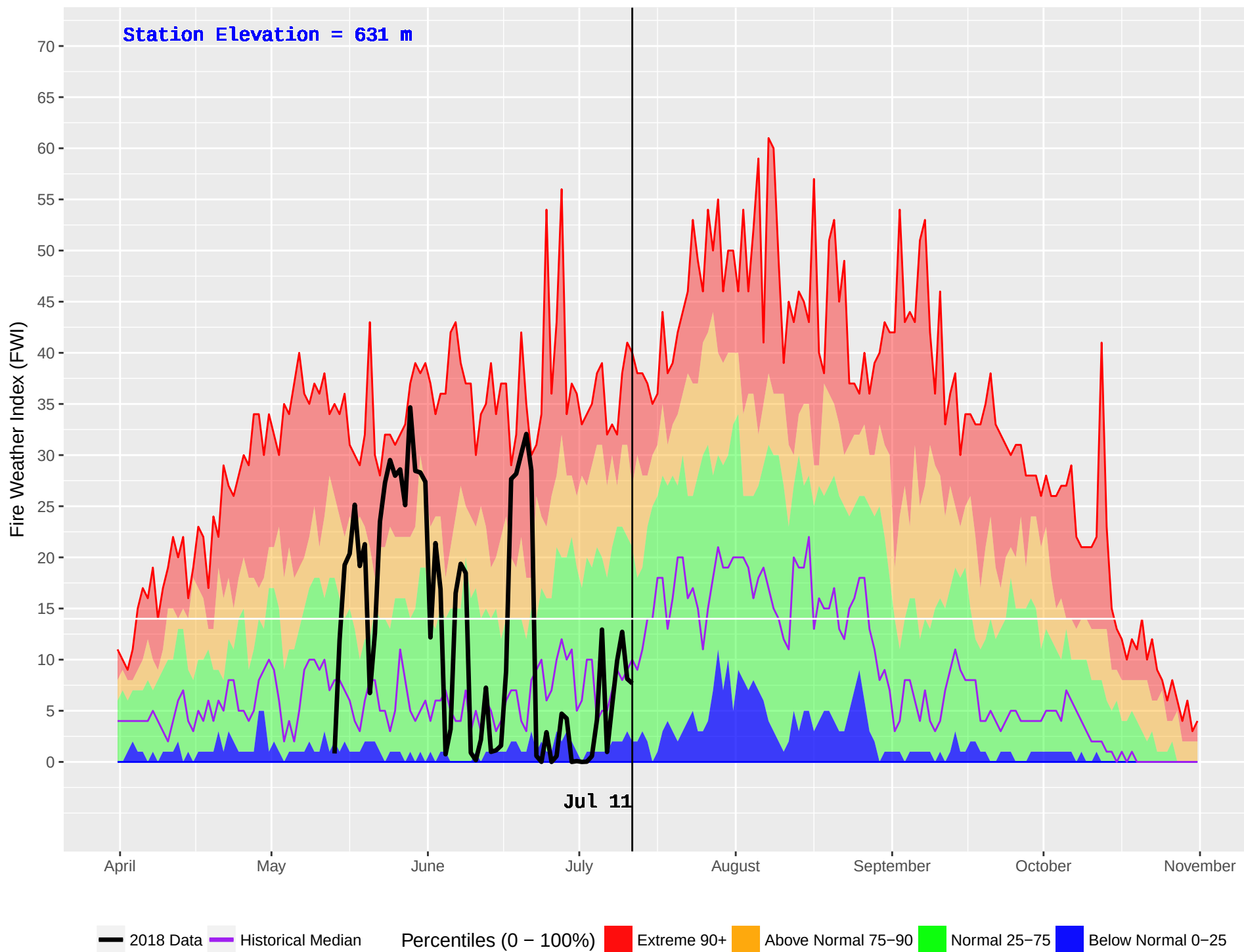
EAST BARRIERE (243) : Historical (1978–2016) and Current (2018) Noon Fire Weather Index (FWI)
