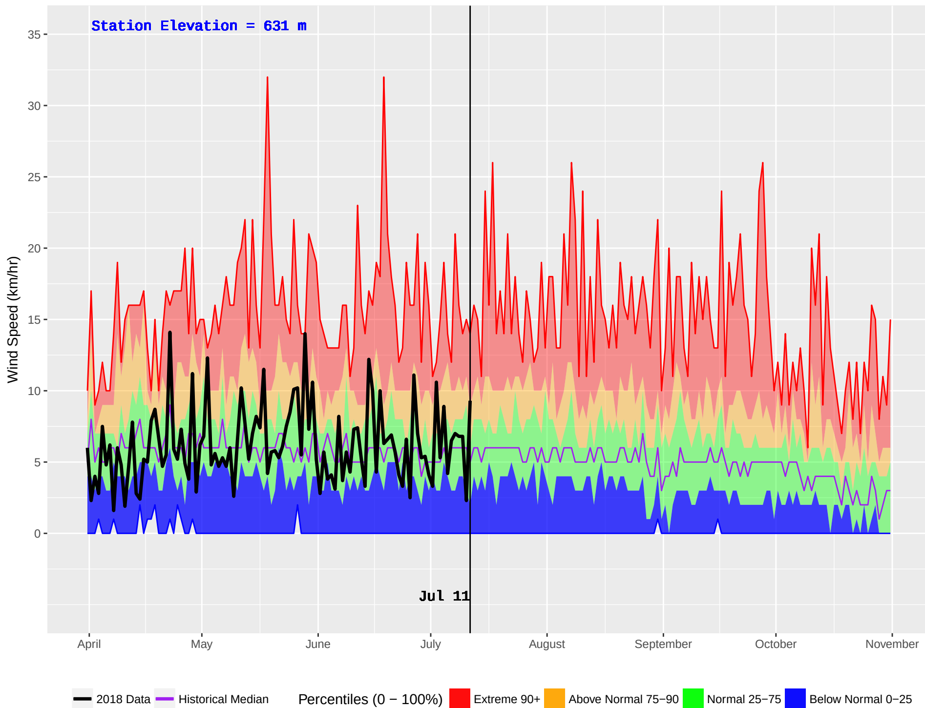
EAST BARRIERE (243) : Historical (1978–2016) and Current (2018) Noon Wind Speed
