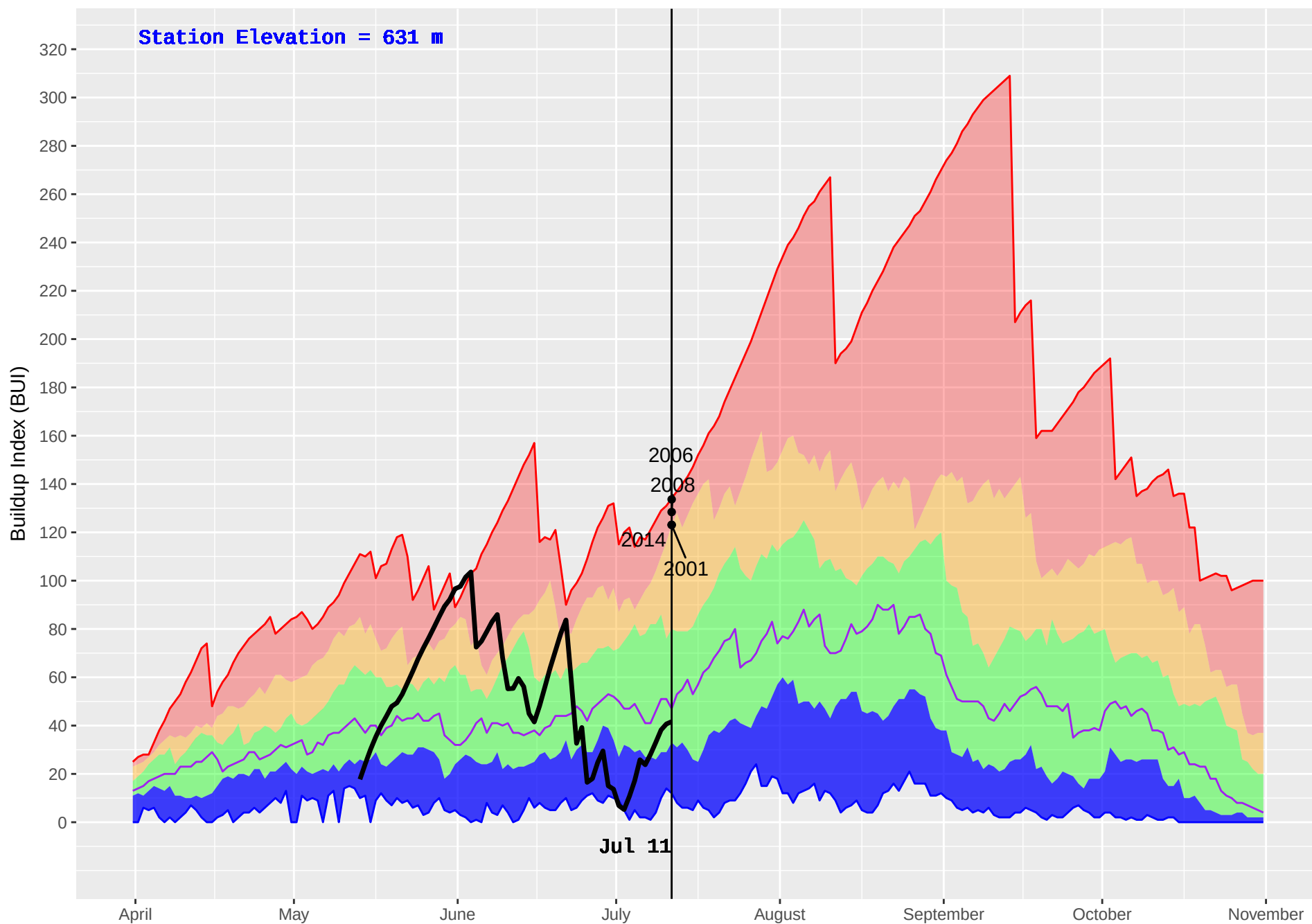
EAST BARRIERE (243) : Historical (1978–2016) and Current (2018) Noon Buildup Index (BUI)
