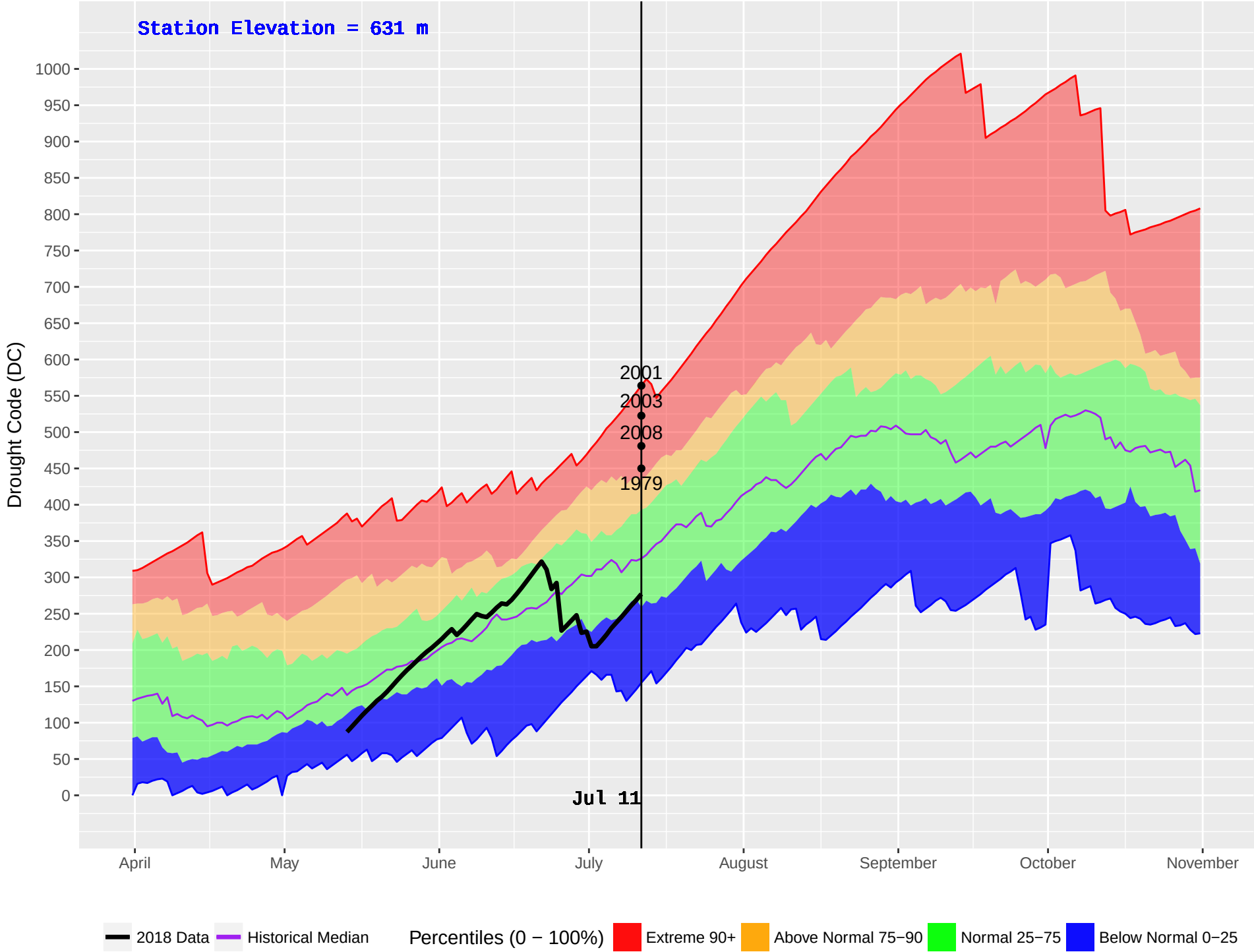
EAST BARRIERE (243) : Historical (1978–2016) and Current (2018) Noon Drought Code (DC)
